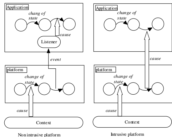
Figure 12 : Modes of interaction between platform and application
