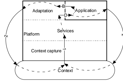
Figure 17 : Intrusive adaptation model
