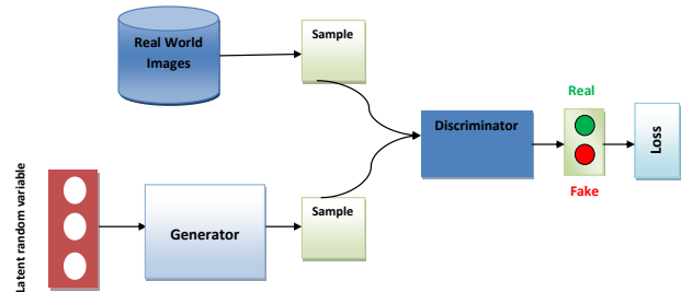
Fig 2: A Plain GAN Schematic Diagram
